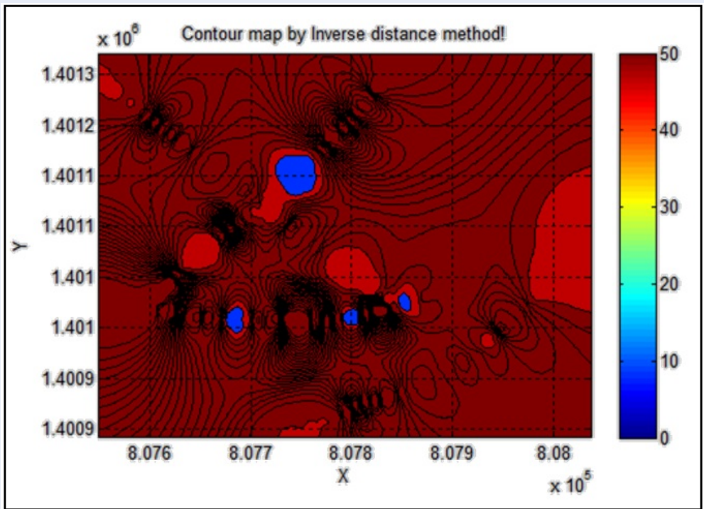
Figure 10: The resistivity contour of layer depth -25m with modify value <50 Ω.m
