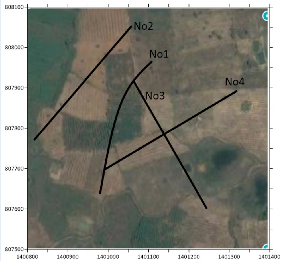
Figure 2: The location of VES stations
