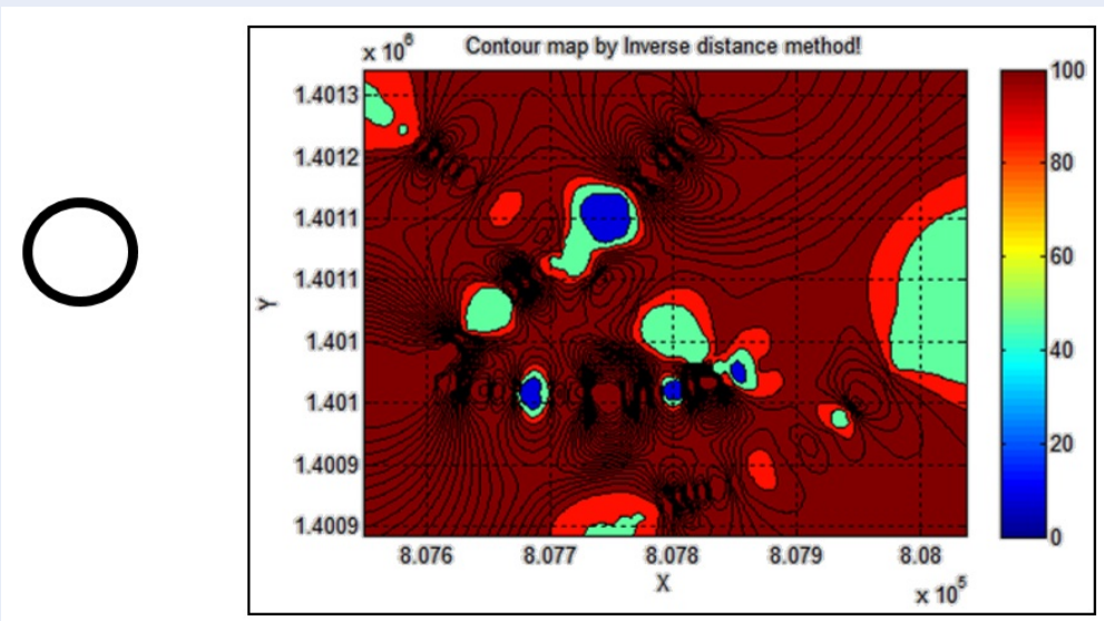
Figure 9: The resistivity contour map of layer depth -25m with modify value <100 Ω.m
