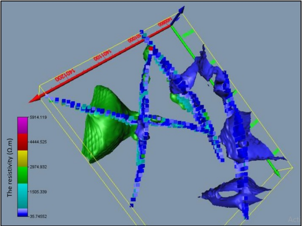
Figure 5: 3-D imaging profile of resistivity isosurface at 250 and 2240 Ω.m
