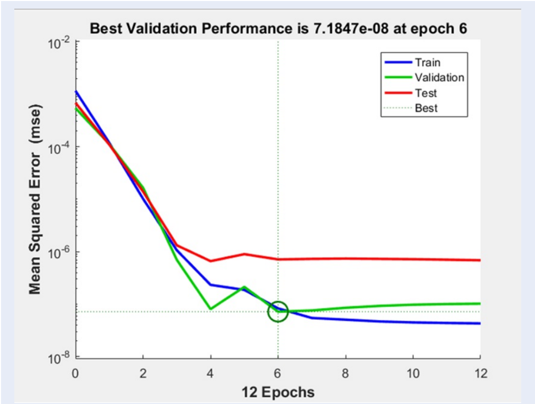
Figure 11: Graph shows the MSE values when applying the original normalized datasets to the same artificial neural network
