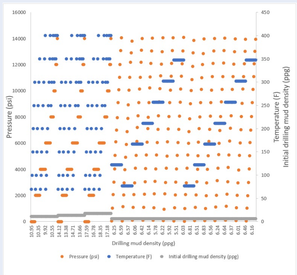
Figure 1: The data collected from the works of McMordie et al. (1982) and Demirdal & Cunha (2009) were used in this research for the nonlinear function
