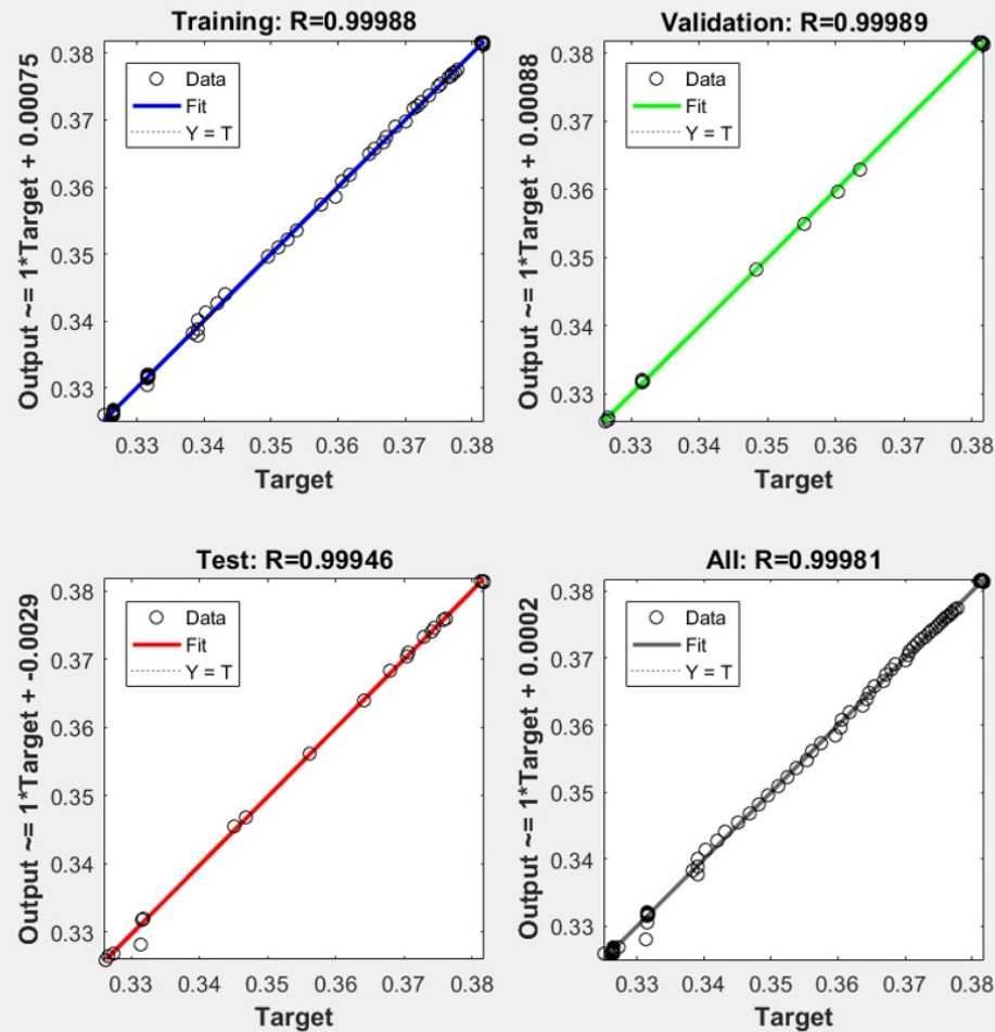
Figure 13: Graph shows the R values when applying the original normalized datasets to the artificial neural network with one hidden layer
