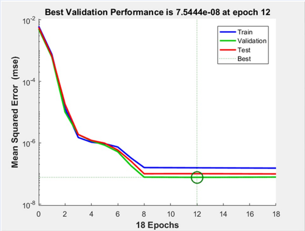
Figure 12: Graph shows the MSE values when applying the original normalized datasets to the artificial neural network with one hidden layer
