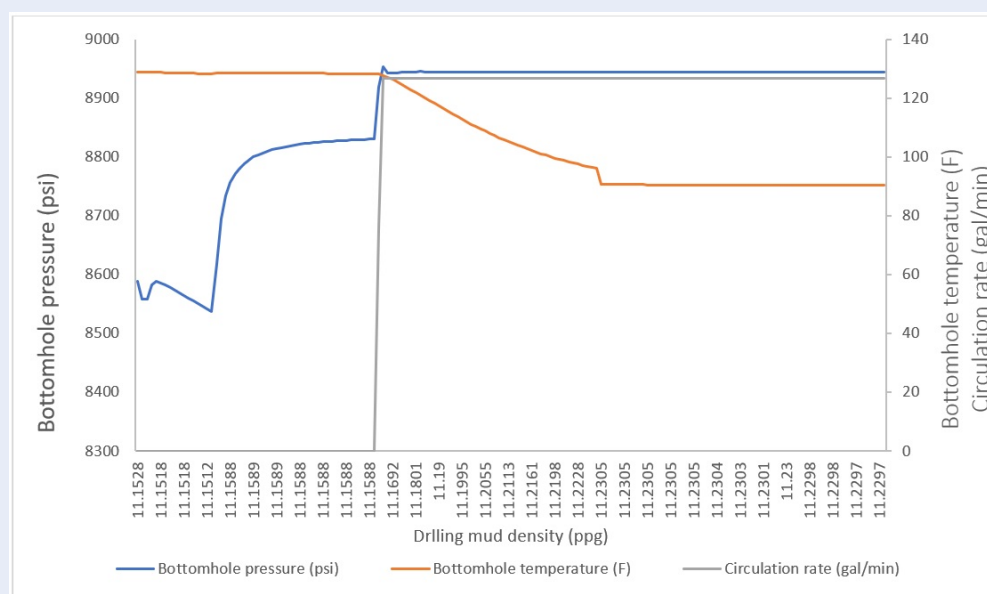
Figure 6: Input data used in this study to build the artificial neural network was provided by Schlumberger in Drilbench software's tutorial
