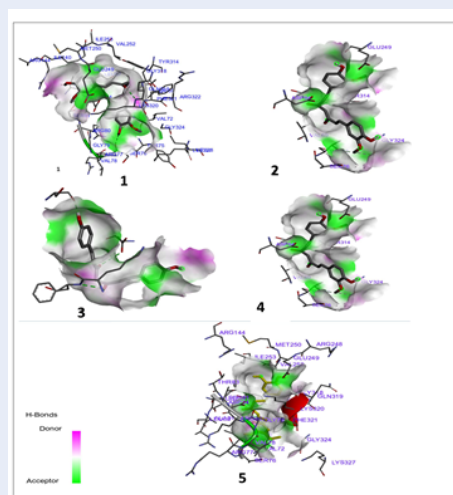
Figure 5: Pocket site with H-Bonds of compounds and the receptor. [Source: Authors]
