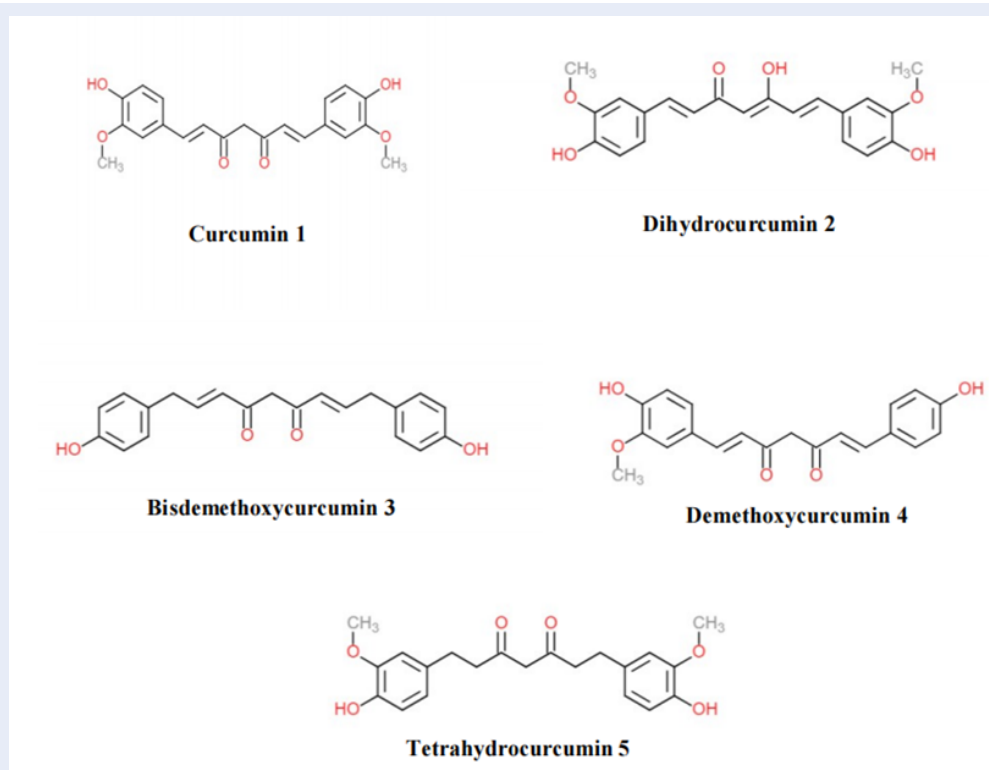
Figure 1: 2D structures for the study of compounds (1–5). [Source: Authors]
