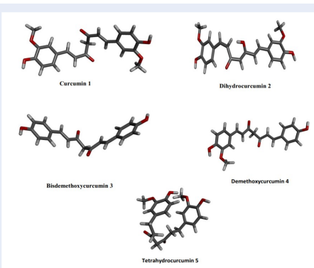
Figure 3: The optimized structure of compounds under study. [Source: Authors]
