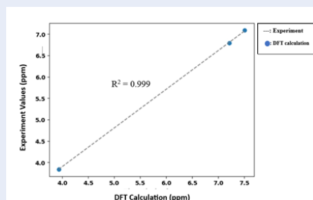
Figure 2: NMR values in theoretical and experimental study for the compound 2. [Source: Authors]
