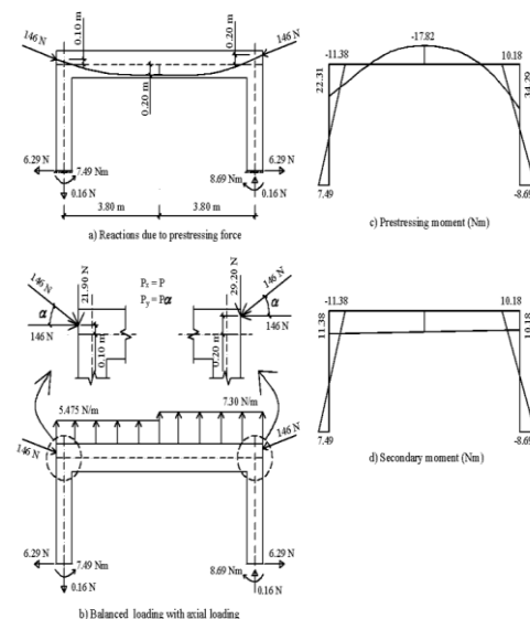
Figure 13. Analyzing single-span frame using load balancing method 13
