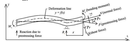
Figure 14. The equilibrium of prestressed member with large tendon profile sag [Source: The Authors]
