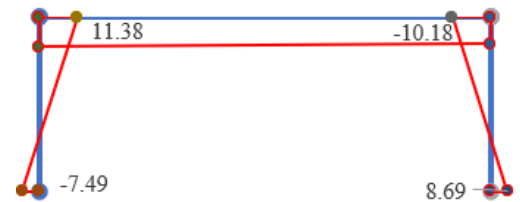
Figure 11. The secondary moment diagram of frame (Nm) [Source: The Authors]
