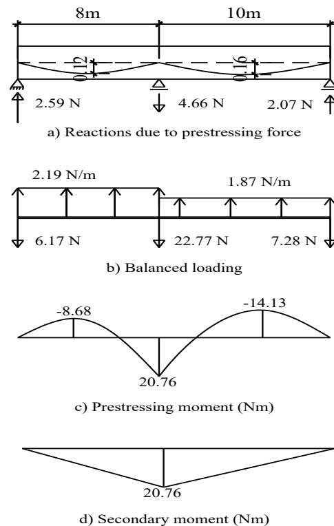
Figure 12. Analyzing two-span beam using load balancing method [Source: The Authors]
