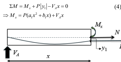
Figure 3. The equilibrium of the left segment from point A [Source: The Authors]
